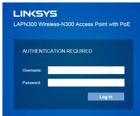
Figure 1: Password Dialog
