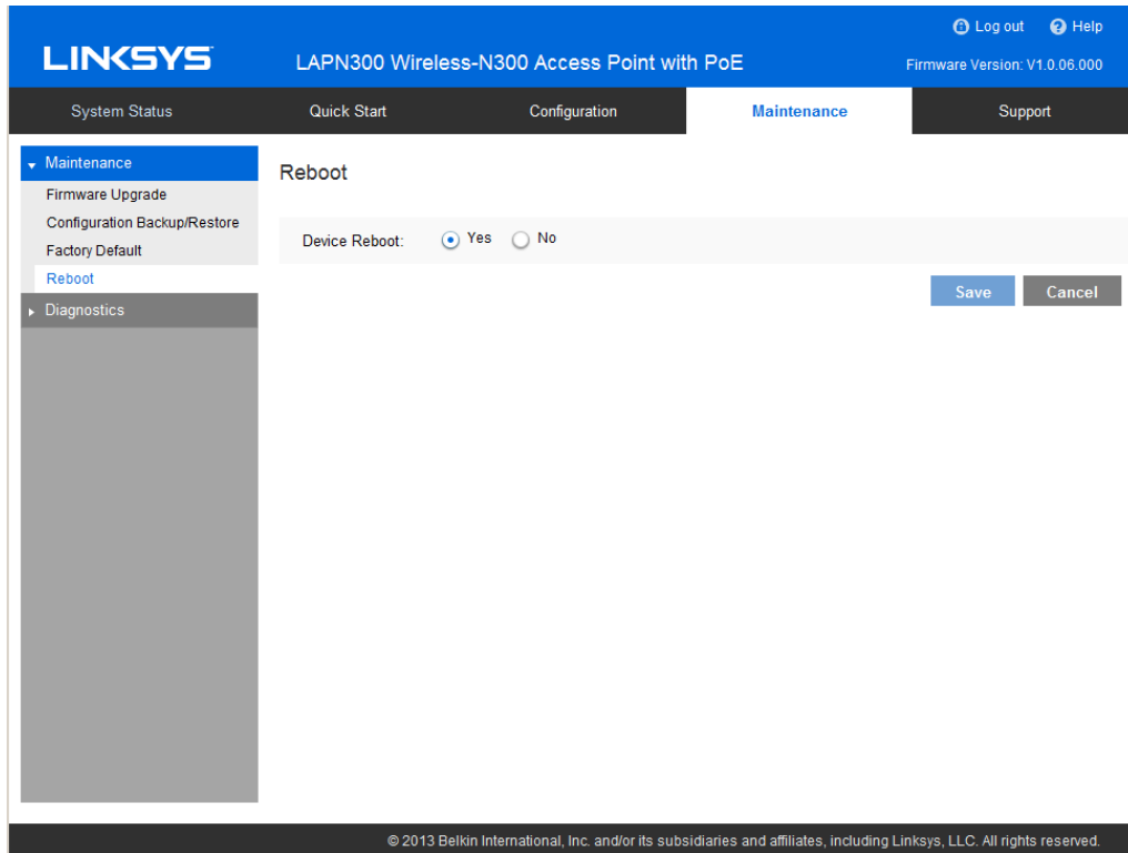
Figure 41: Reboot Screen
