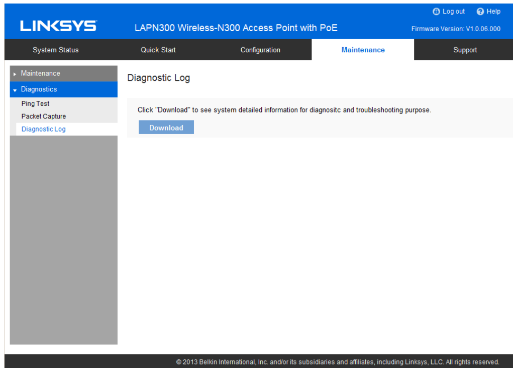
Figure 44: Diagnostic Screen
