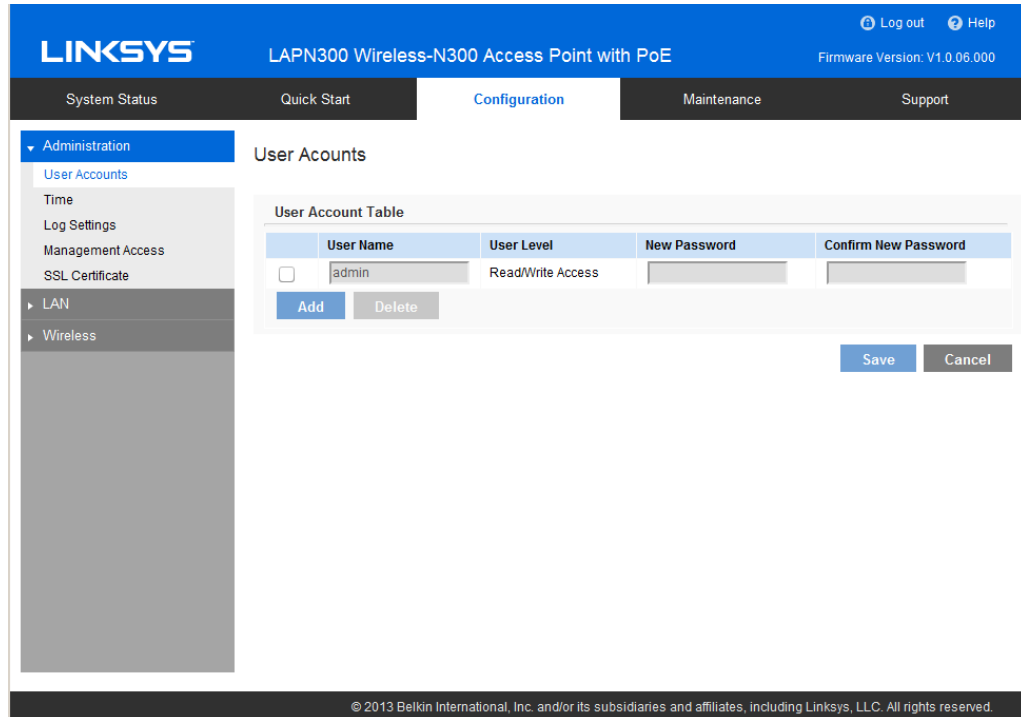
Figure 9: User Accounts
