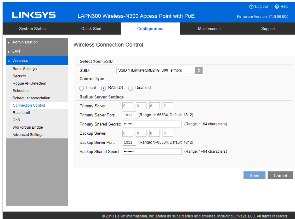
Figure 27: Connection Control Screen
