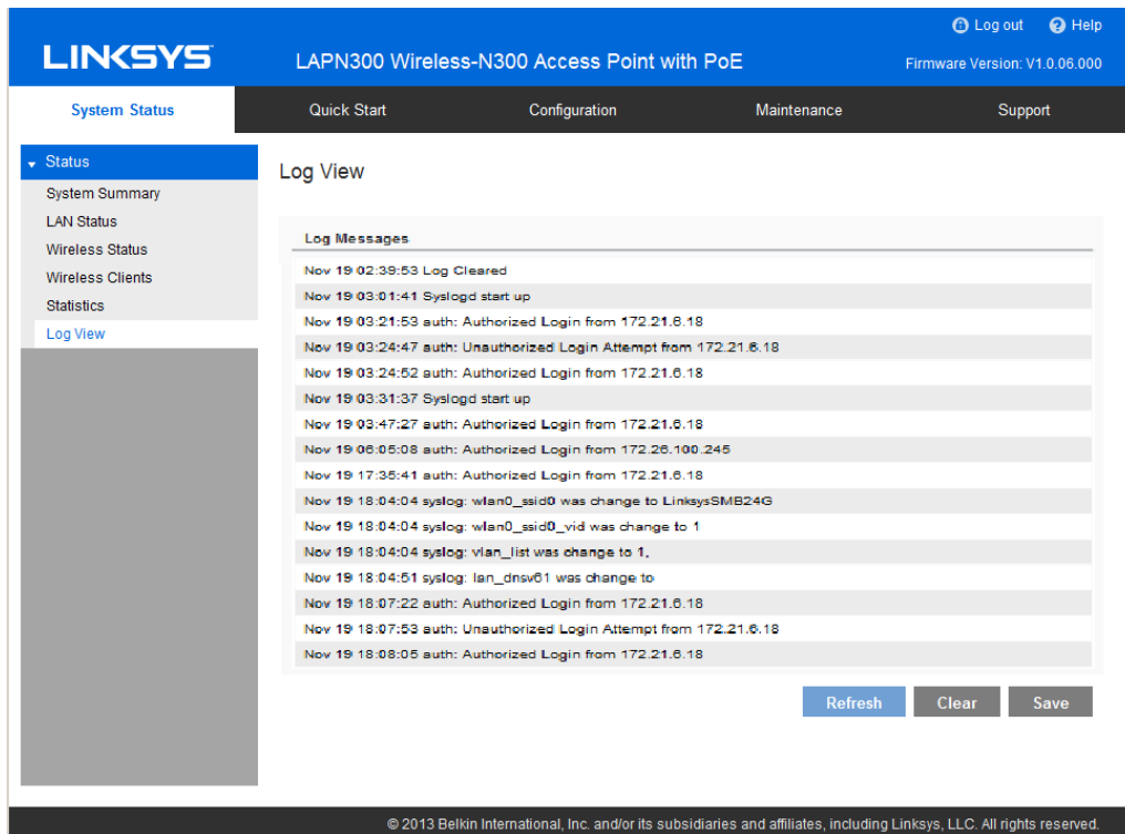
Figure 37: Log View Screen
