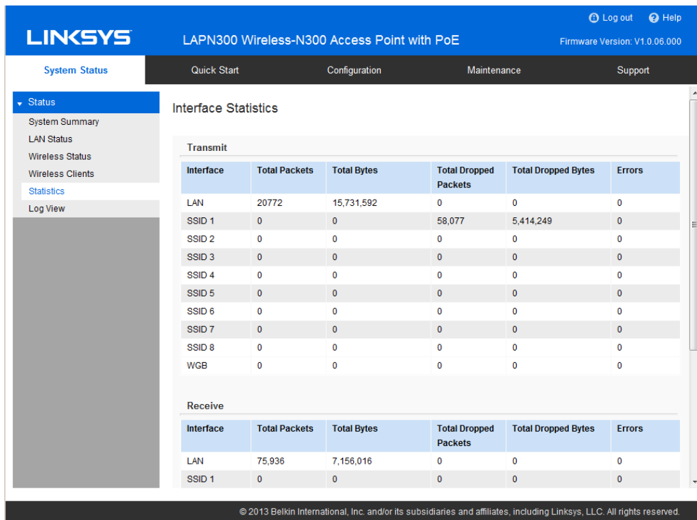
Figure 36: Statistics Screen
