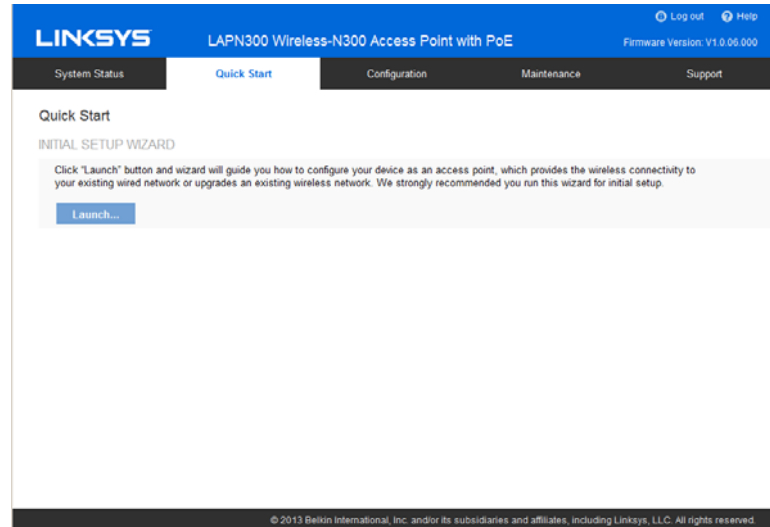
Figure 2: Setup Wizard
